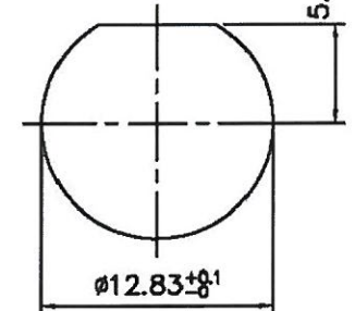
RECOMMEND PANEL HOLE
