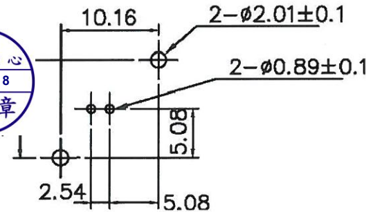
RECOMMENDED PCB HOLE
